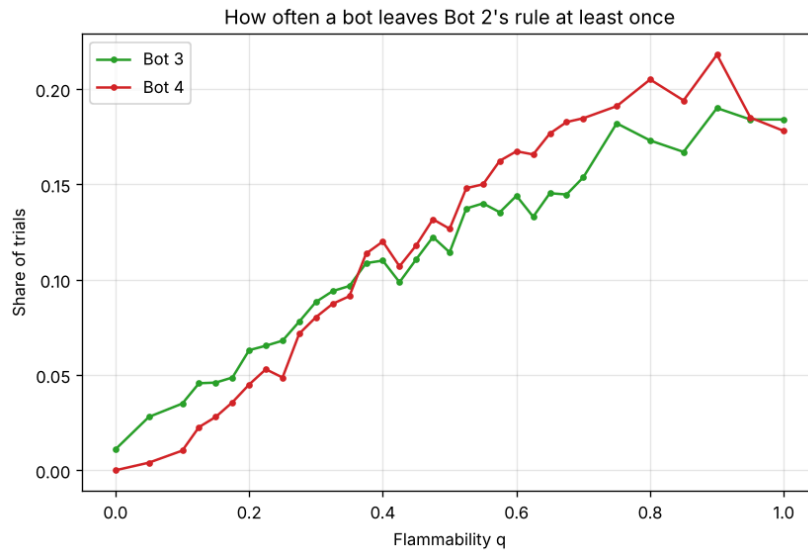
Figure 4: Share of trials in which Bot 3 or Bot 4 makes at least one move that Bot 2’s rule (step along some shortest fire-free path) could not have made.
