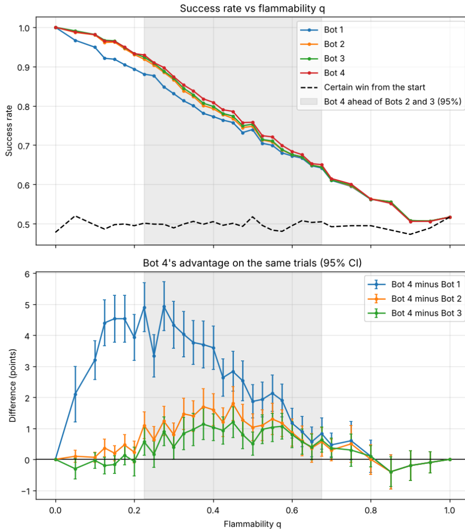
Figure 3: Top: success rate against flammability q for every bot, with the share of trials that are certain wins from the start dashed. Bottom: Bot 4's success rate minus each other bot's on the same trials, in percentage points, with 95% confidence intervals. The shaded band is where Bot 4 beats both Bot 2 and Bot 3 with 95% confidence.
