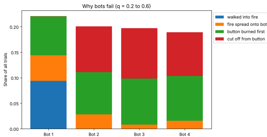
Figure 5: Why the bots fail, as a share of all trials at q from 0.2 to 0.6.
